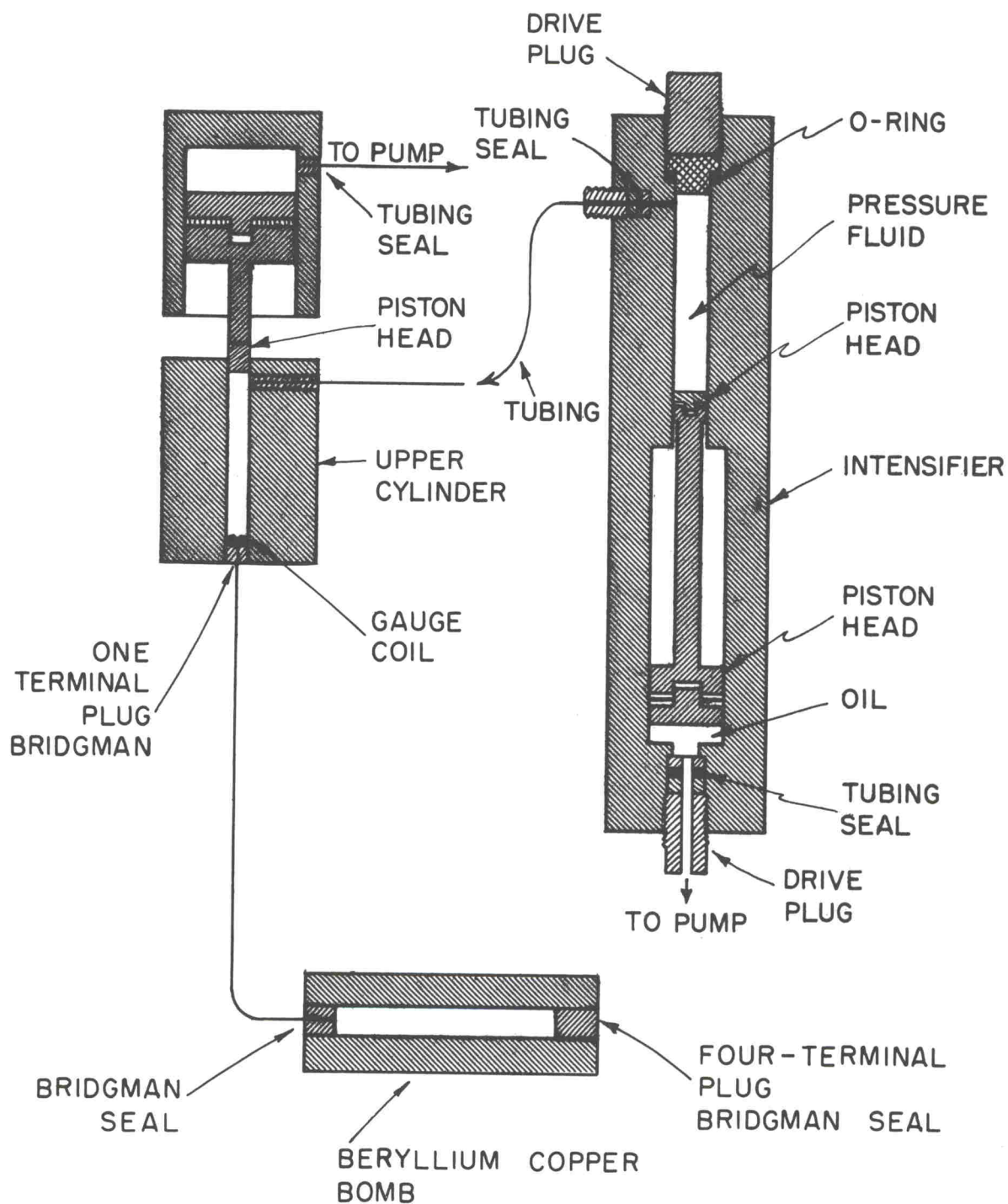
FIG. 2-3 SCHEMATIC DIAGRAM OF 15,000 kg/cm 2 HIGH PRESSURE APPARATUS
